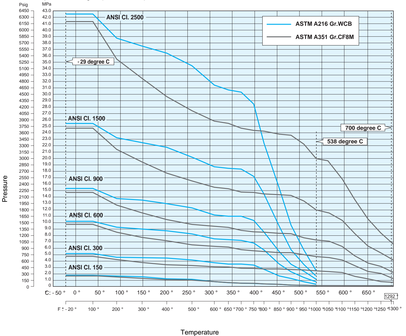
Pressure-Temperature Ratings (ANSI B 16.34)
