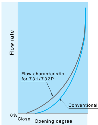
Flow characteristic
